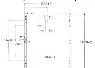
Drawing of 310Wp - 330 Wp Module
